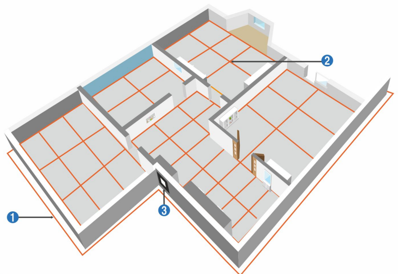
View of Network of APPROTECH Porous Pipes
